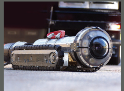
CUES® Digital Universal Camera (DUC)
